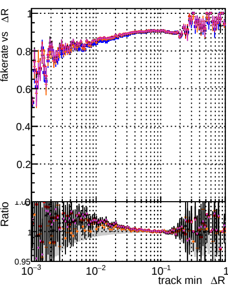
Fake rate vs \Delta R (track, jet) Legend: DOM CKFit 1000evt, DOM CKFit 10000evt, DOM CKFit 100000evt, DOM TESTOLHIT 10000evt, DOM TESTOLHIT 100000evt, DOM TESTOLHIT 500000evt
