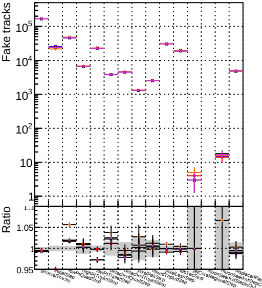
Number Line Style Label 1 Black line with cross-ticks DOM MKFITREFIT 1000evt 2 Orange line with cross-ticks DOM TESTOLHIT 1000evt 3 Purple line with cross-ticks DOM TESTOLHIT 1000evt-50000t
