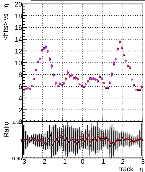
mean hits vs \eta DOM CKFEE1 1000evt DOM CKFEE1 1000evt DOM CKFEE1 1000evt DOM TESTOLHIT 1000evt DOM TESTOLHIT 1000evt-50000t
