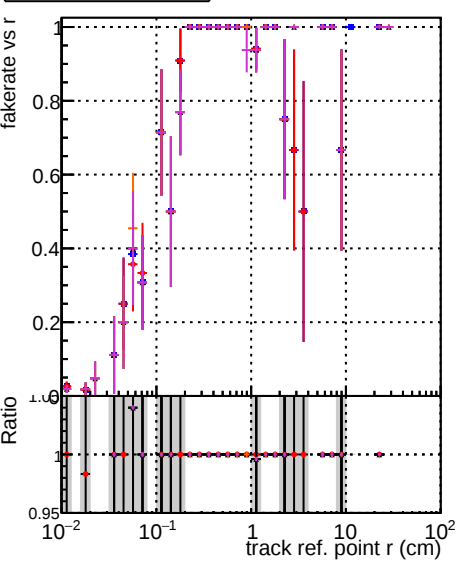
Fake rate vs vertpos Legend: DOM CKFit 1000evt, DOM CKFit 10000evt, DOM CKFit 100000evt, DOM TESTOLHIT 10000evt, DOM TESTOLHIT 50000evt
