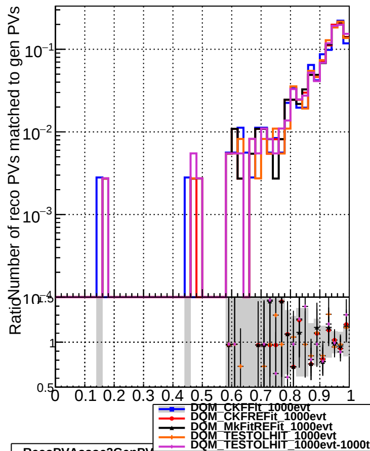
RecoPVAssoc2GenPVmatched_missing
