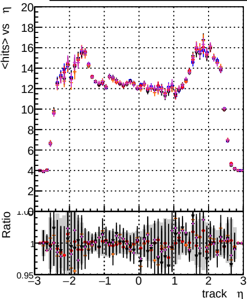
mean hit DOM CKFFIT_1000evt DOM CKFFIT_1000evt DOM CKFFIT_1000evt DOM TESTOLHIT_1000evt DOM TESTOLHIT_1000evt-1000t
