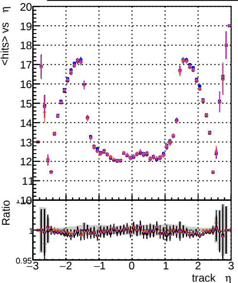
mean hits vs \eta DOM CKFFIT_1000evt DOM CKFFIT_1000evt DOM CKFFIT_1000evt DOM TESTOLHIT_1000evt DOM TESTOLHIT_1000evt-1000t
