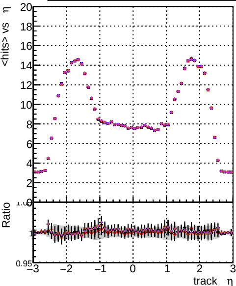
mean hits vs \eta DOM CKFEE1_1000evt DOM CKFEE1_1000evt DOM CKFEE1_1000evt DOM TESTOLHIT_1000evt DOM TESTOLHIT_1000evt-1000t
