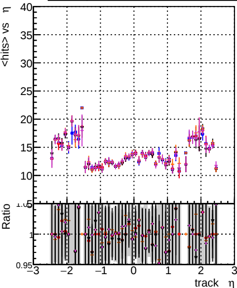
mean hit \eta DOM CKFit 1000evt DOM CKFit 10000evt DOM CKFit 100000evt DOM TESTOLHIT 1000evt DOM TESTOLHIT 1000000
