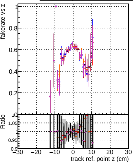
Fake rate vs track ref. point z
