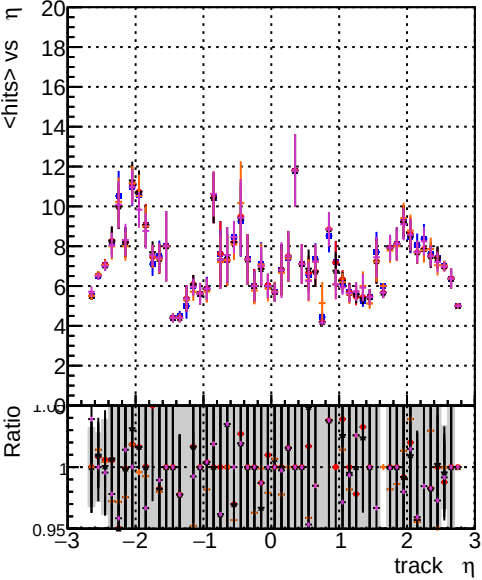
mean hits vs \eta DOM CKFit 1000evt DOM CKFit 10000evt DOM CKFit 100000evt DOM TESTOLHIT 1000evt DOM TESTOLHIT 10000evt-1000t
