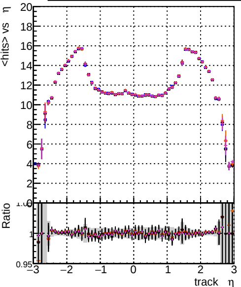
mean hits vs \eta DOM CKFIT 1000evt DOM CKREFIT 1000evt DOM CKFIT 10000evt DOM TESTOLHIT 1000evt DOM TESTOLHIT 1000evt-1000t
