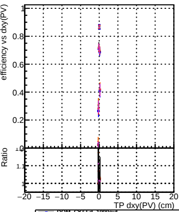
Efficiency vs Dxy(PV) Legend: DOM_CKFit_1000evt DOM_CKFit_1000evt DOM_MkFit_1000evt DOM_TESTOLHIT_1000evt DOM_TESTOLHIT_1000evt-1000t
