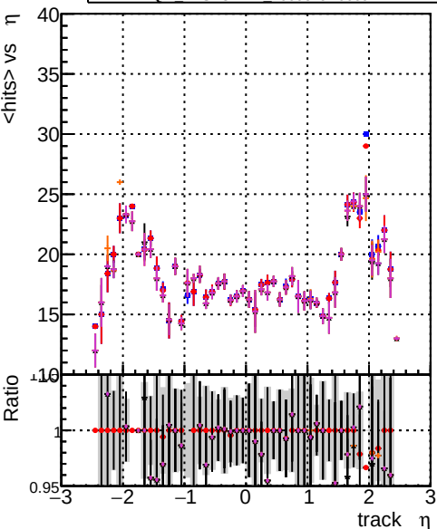
mean hit DOM CKFEE1 1000evt DOM CKFEE2 1000evt DOM CKFEE3 1000evt DOM TESTOLHIT 1000evt DOM TESTOLHIT 1000evt-1000t
