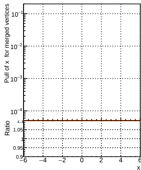
RecoAllAssoc2GenMatchedMerged_PulIX
