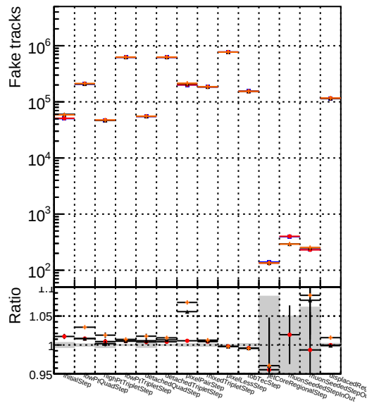
Number of tracks vs collection Legend: DOM_CKFit_1000evt (blue circles) DOM_CKFit_1000evt (red circles) DOM_MkFitREFit_1000evt (black triangles) DOM_TESTOLHIT_1000evt (orange squares)
