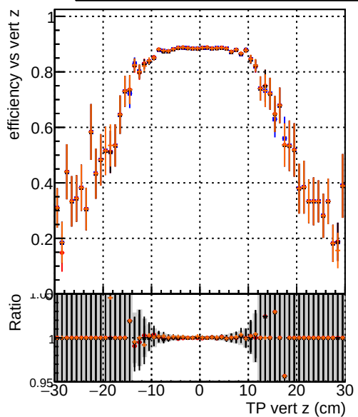
Efficiency vs. TP vert z (cm) Legend: - DOM_CKFFit_1000evt (blue circles) - DOM_CKFREFit_1000evt (red circles) - DOM_MkFitREFit_1000evt (black crosses) - DOM_TESTOLHIT_1000evt (orange circles)
