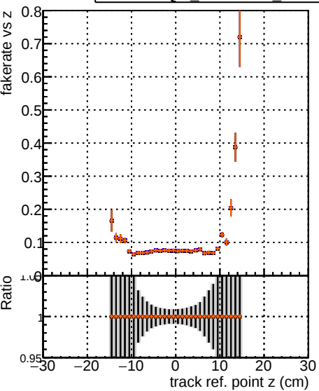
Fake rate vs verpos Legend: DOM CKF test 1000evt (blue line with circles) DOM CKF test 1000evt (red line with circles) DOM CKF test 1000evt (black line with circles) DOM CKF test 1000evt (orange line with circles)
