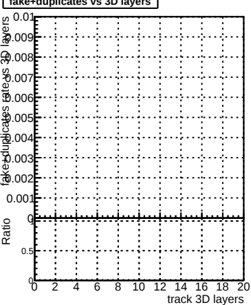
fake+duplicates rate vs 3D layers
