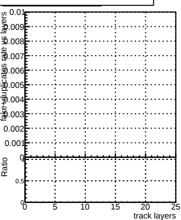
fake+duplicates rate vs TP layers
