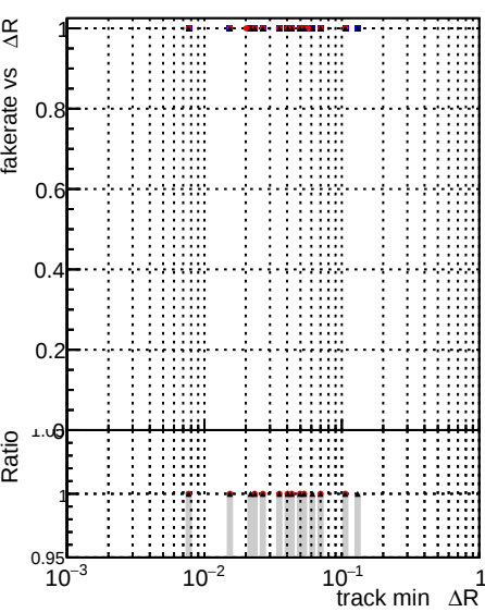
Fake rate vs \Delta R(\text{track, jet}) Legend: DOM CKFFit 1000evt DOM CKFREFit 1000evt DOM NOTESTCKF 1000evt
