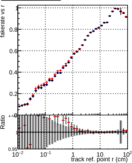
Fake rate vs v Legend: DOM CKFFit 1000evt (blue squares) DOM CKFREFit 1000evt (red circles) DOM NOTESTCKF 1000evt (black crosses)
