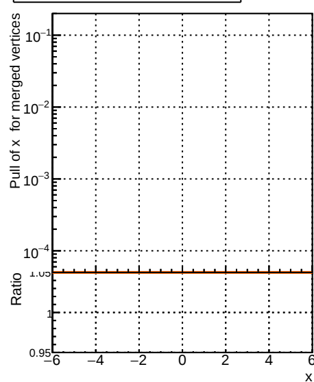
RecoAllAssoc2GenMatchedMerged_PulIX
