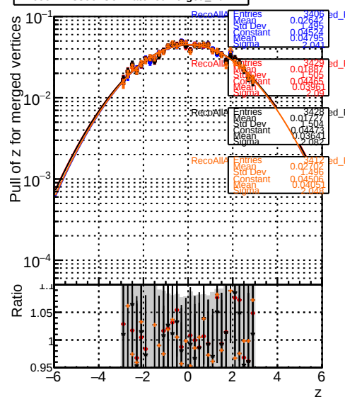
RecoAllAssoc2GenMatchedMerged_PulIZ
