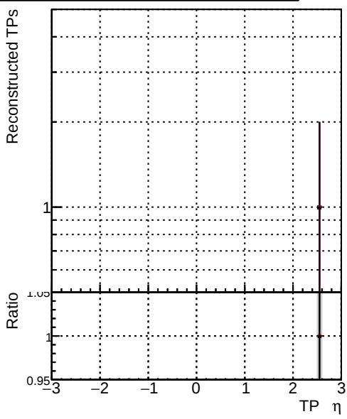
Legend: DQM_CKF-testLowPt_1000evt (blue line with dots), DQM_CKFFit-testLowPt_1000evt (red line with dots), DQM_mkFitREFit-testLowPt_1000evt (black line with dots)
