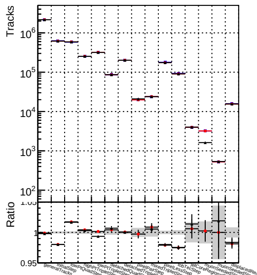
Number of tracks vs collection Legend: - DQM_CKF-testLowPt_1000evt (Blue line with circles) - DQM_CKFFit-testLowPt_1000evt (Red line with circles) - DQM_mkFitREFit-testLowPt_1000evt (Black line with circles)
