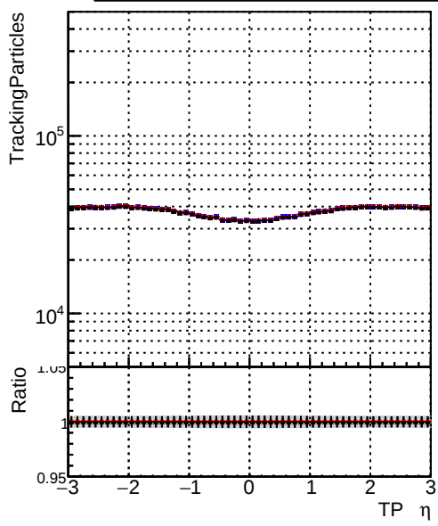
Legend for all plots: DQM_CKF-testLowPt_1000evt (Blue line with dots) DQM_CKFFit-testLowPt_1000evt (Red line with dots) DQM_mkFitREFit-testLowPt_1000evt (Black line with dots)
