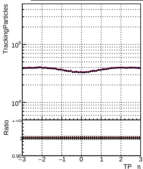
N of simulated tracks vs eta Legend: DQM_CKF-testLowPt_1000evt (blue line with circles) DQM_CKFREFit-testLowPt_1000evt (red line with circles) DQM_mkFitREFit-testLowPt_1000evt (black line with circles)
