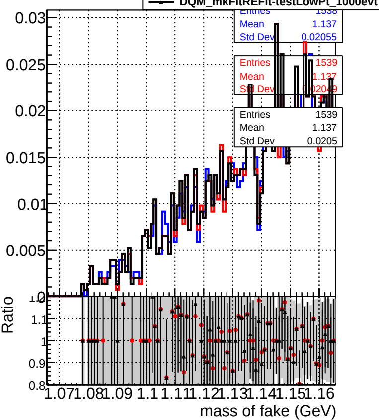
Mass of fake Lambda
