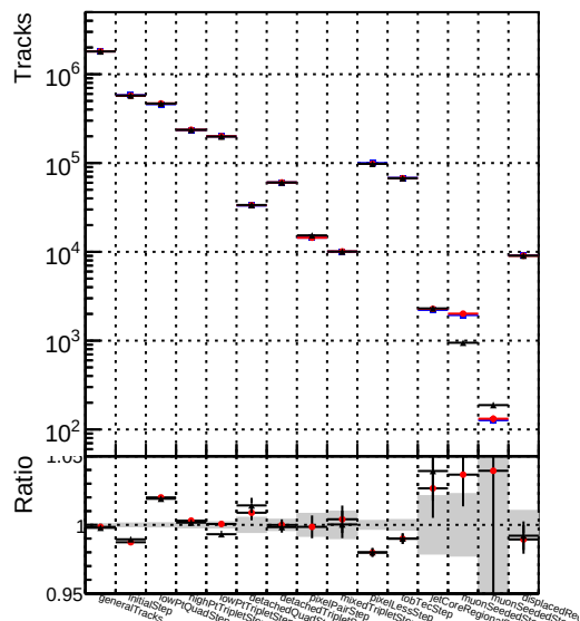
Number of tracks vs collection Legend: DQM_CKF-test_1000evt (blue) DQM_CKFREFit-test_1000evt (red) DQM_mkFitREFit-test_1000evt (black)
