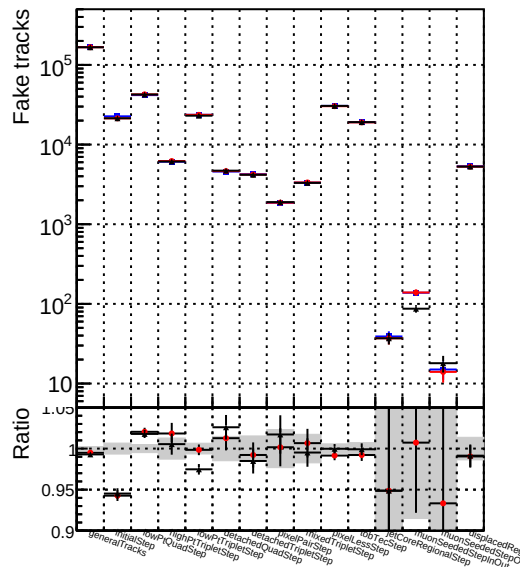
Number of tracks vs collection Legend: DQM_CKF-test_1000evt (blue) DQM_CKFREFit-test_1000evt (red) DQM_mkFitREFit-test_1000evt (black)
