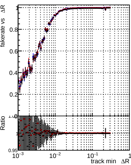
Legend: DOM_CKF-test_1000evt (blue squares), DOM_CKFREFit-test_1000evt (red circles), DOM_mkFitREFit-test_1000evt (black triangles)
