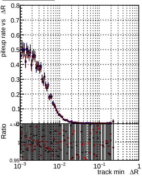
Legend: DOM_CKF-test_1000evt (blue squares), DOM_CKFREFit-test_1000evt (red circles), DOM_mkFitREFit-test_1000evt (black triangles)
