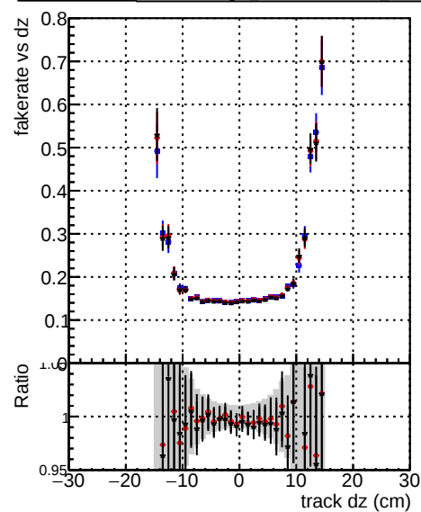
Fake rate vs dz Legend: DOM CKE fit-test 1000evt (blue line with circles) DOM CKE fit-test 1000evt (red line with circles) DOM mkr fit-test 1000evt (black line with circles)
