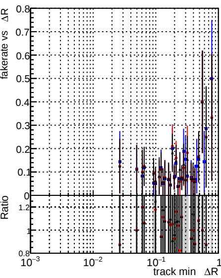
Fake rate vs ΔR(track, jet) DOM_CKF-test_1000evt DOM_CKFREFit-test_1000evt DOM_mkFitREFit-test_1000evt
