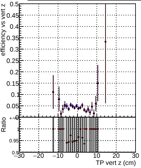
Efficiency vs TP vert z (cm) Legend: DQM_CKF-test_1000evt (blue dots) DQM_CKFREFit-test_1000evt (red dots) DQM_mkFitREFit-test_1000evt (black dots)
