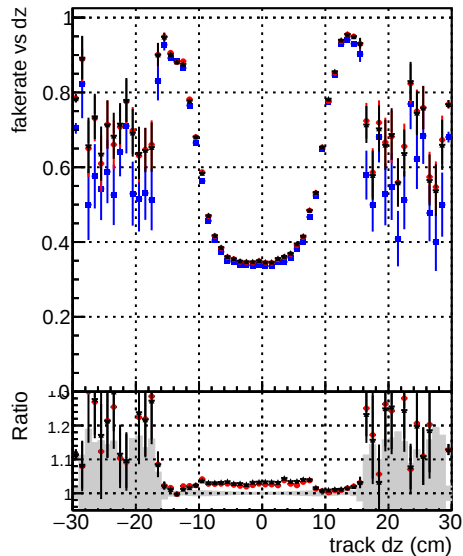
DOM original_step2_tbar-phase1-newgeom pixelCPE_step2_tbar-phase1-newgeom DOM pixelCPEAndCh12_step2_tbar-phase1-newgeom
