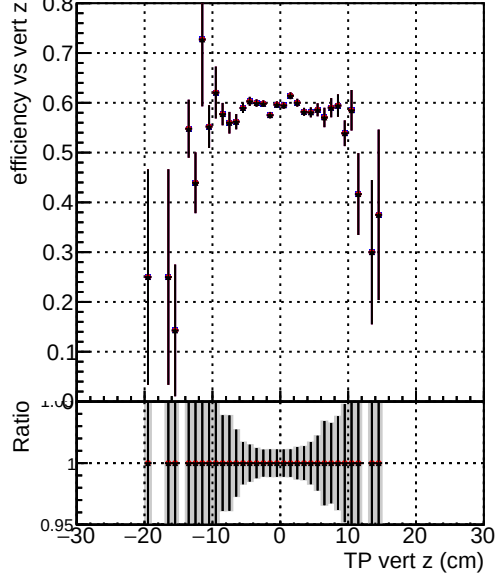
Efficiency vs. TP vert z —●— DQM_original_step2_ttbar-phase1-newgeom —●— DQM_pixelCPE_step2_ttbar-phase1-newgeom —●— DQM_pixelCPEAndChi2_step2_ttbar-phase1-newgeom
