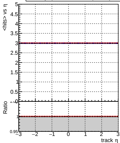
mean hits — DQM_original_step2_ttbar-phase1-newgeom — DQM_pixelCPE_step2_ttbar-phase1-newgeom — DQM_pixelCPEAndChi2_step2_ttbar-phase1-newgeom
