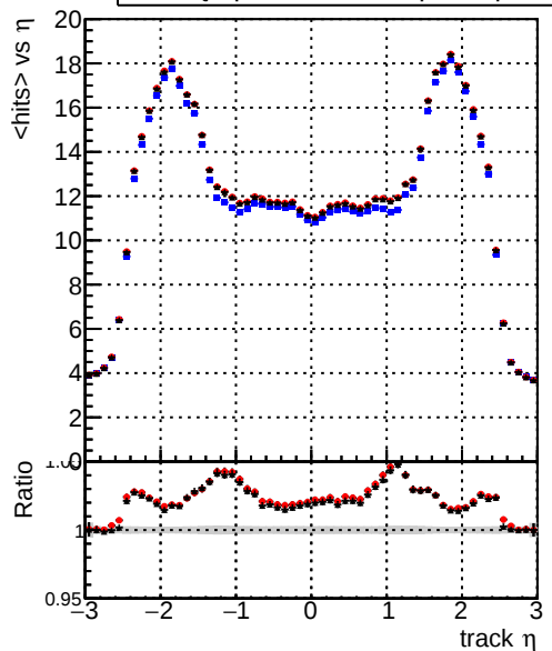
DQM_original_step2_ttbar-phase1-newgeom DQM_pixelCPE_step2_ttbar-phase1-newgeom DQM_pixelCPEAndChi2_step2_ttbar-phase1-newgeom mean hits
