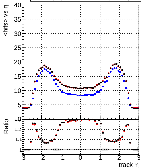
DQM_original_step2_ttbar-phase1-newgeom DQM_pixelCPE_step2_ttbar-phase1-newgeom DQM_pixelCPEAndChi2_step2_ttbar-phase1-newgeom mean hits
