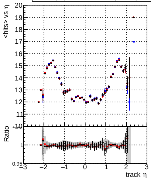
mean hits vs \eta DQM_original_step2_ttbar-phase1-newgeom DQM_pixelCPE_step2_ttbar-phase1-newgeom DQM_pixelCPEAndChi2_step2_ttbar-phase1-newgeom
