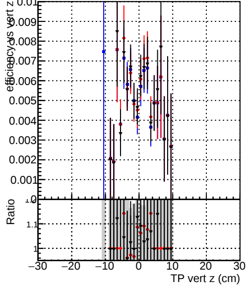
Efficiency vs. sim PV z —●— DQM_original_step2_ttbar-phase1-newgeom —●— DQM_pixelCPE_step2_ttbar-phase1-newgeom —●— DQM_pixelCPEAndChi2_step2_ttbar-phase1-newgeom
