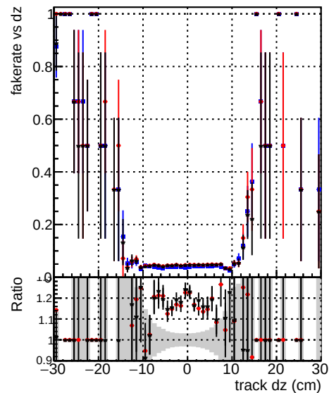
DOM pixelCPE_step2 ttbar-phase1-newgeom DOM pixelCPEAndChi2_step2 ttbar-phase1-newgeom
