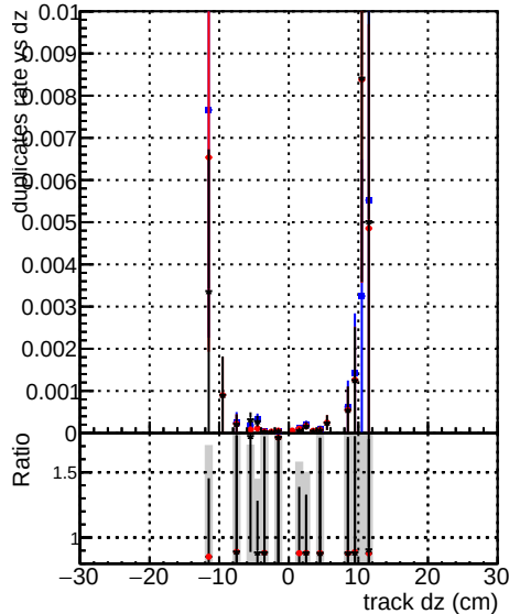
DOM pixelCPE_step2 ttbar-phase1-newgeom DOM pixelCPEAndChi2_step2 ttbar-phase1-newgeom
