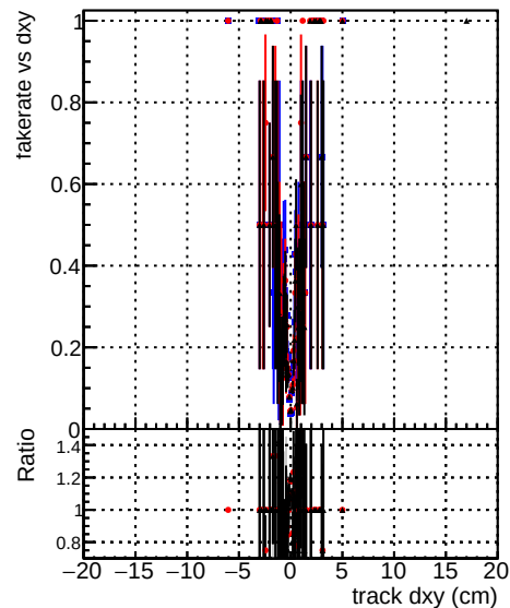
DOM original step2 ttbar-phase1-newgeom DOM-nix@ICPE step2 ttbar-phase1-newgeom
