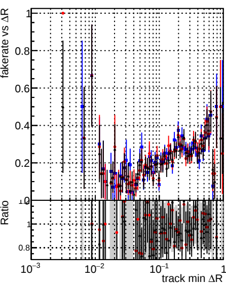
Fake rate vs \Delta R (track, jet) DQM_original_step2_ttbar-phase1-newgeom DQM_pixelCPE_step2_ttbar-phase1-newgeom DQM_pixelCPEAndChi2_step2_ttbar-phase1-newgeom
