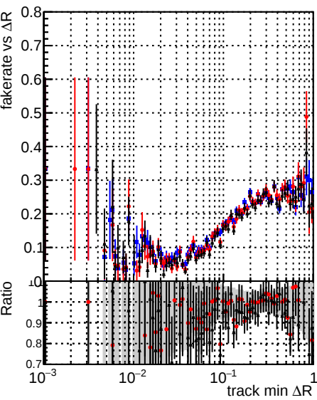
Fake rate vs \Delta R(\text{track, jet}) Legend: DQM_original_step2_ttbar-phase1-newgeom (blue squares) DQM_pixelCPE_step2_ttbar-phase1-newgeom (red circles) DQM_pixelCPEAndChi2_step2_ttbar-phase1-newgeom (black triangles)
