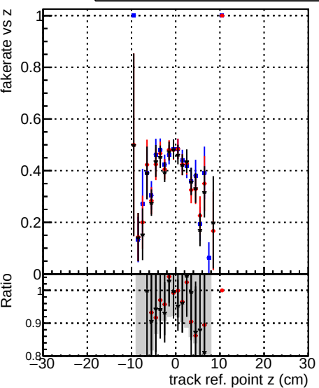
Fake rate vs verpos — DQM_original_step2_ttbar-phase1-newgeom — DQM_pixelCPE_step2_ttbar-phase1-newgeom — DQM_pixelCPEAndChi2_step2_ttbar-phase1-newgeom
