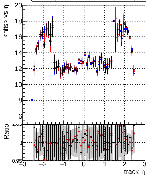
mean hit — DQM_original_step2_ttbar-phase1-newgeom — DQM_pixelCPE_step2_ttbar-phase1-newgeom — DQM_pixelCPEAndChi2_step2_ttbar-phase1-newgeom
