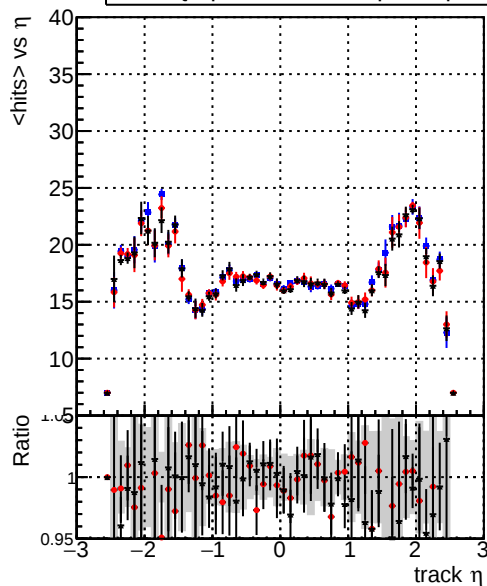
mean hits — DQM_original_step2_ttbar-phase1-newgeom — DQM_pixelCPE_step2_ttbar-phase1-newgeom — DQM_pixelCPEAndChi2_step2_ttbar-phase1-newgeom
