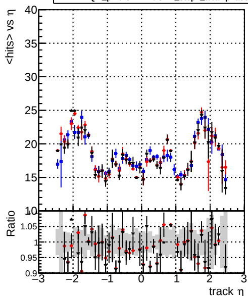
mean hit — DQM_original_step2_ttbar-phase1-newgeom — DQM_pixelCPE_step2_ttbar-phase1-newgeom — DQM_pixelCPEAndChi2_step2_ttbar-phase1-newgeom
