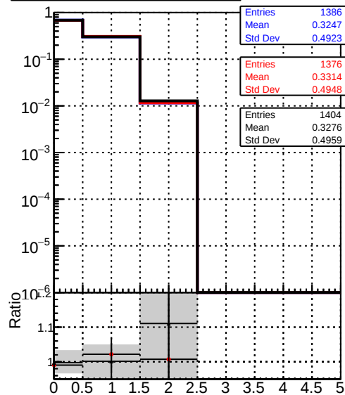
mean hit — DQM_original_step2_ttbar-phase1-newgeom — DQM_pixelCPE_step2_ttbar-phase1-newgeom — DQM_pixelCPEAndChi2_step2_ttbar-phase1-newgeom
