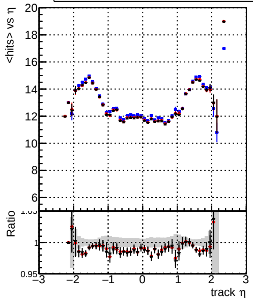
mean hits — DQM_original_step2_ttbar-phase1-newgeom — DQM_pixelCPE_step2_ttbar-phase1-newgeom — DQM_pixelCPEAndChi2_step2_ttbar-phase1-newgeom
