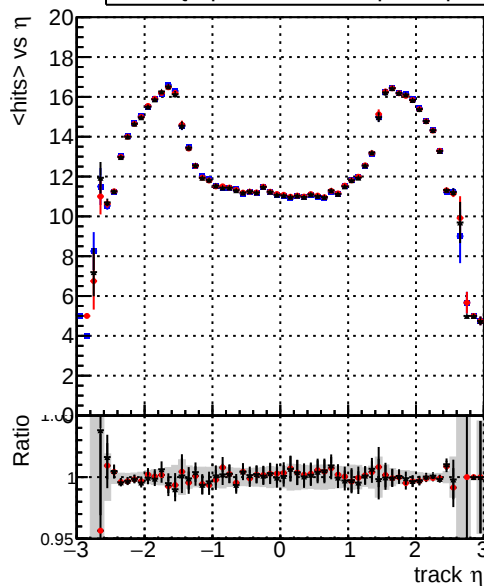
mean hits vs \eta — DQM_original_step2_ttbar-phase1-newgeom — DQM_pixelCPE_step2_ttbar-phase1-newgeom — DQM_pixelCPEAndChi2_step2_ttbar-phase1-newgeom
