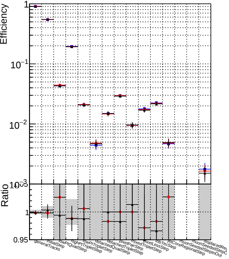
DQM_original_step2_ttbar-phase1-newgeom DQM_pixelCPE_step2_ttbar-phase1-newgeom DQM_pixelCPEAndChi2_step2_ttbar-phase1-newgeom
